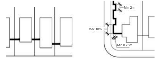
PRIMARY FRONTAGE Structures and Services PRIMARY FRONTAGE
